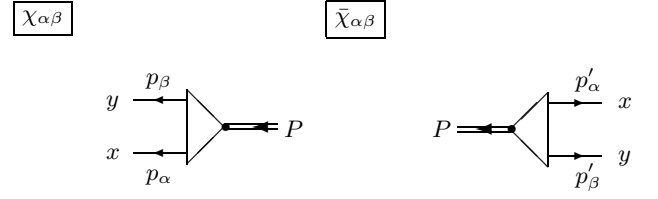
Fig. 14. Momentum definitions in diquark amplitudes.
