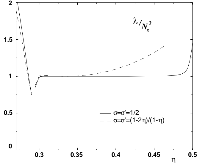
Fig. 4. Dependence of \lambda/N_s^2 on \eta for fixed \sigma = \sigma' = 1/2 (solid) and with \sigma, \sigma' from eq. (3.13) (dashed). The width \gamma_2 is fixed to yield \lambda/N_s^2 = 1 at \eta = 1/3 .
