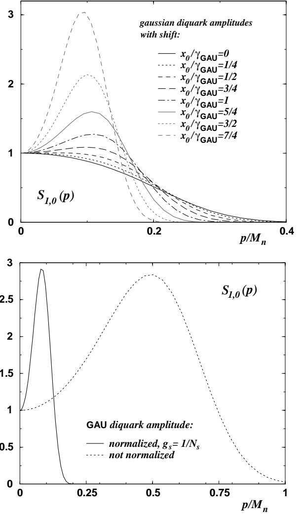
Fig. 7. The moment S_{1,0} for the Gaussian diquark amplitudes of eq. (2.16) with various shifts x_0/\gamma_{\text{Gau}} (top), see Table 2, and a comparison (bottom) of our result for x_0/\gamma_{\text{Gau}} = 19/11 (with m_s = 0.7M_n, m_q = 0.555M_n ) with a result we obtain from using \gamma_{\text{Gau}} = 0.11 \text{ GeV}^2 as in ref. [22].
