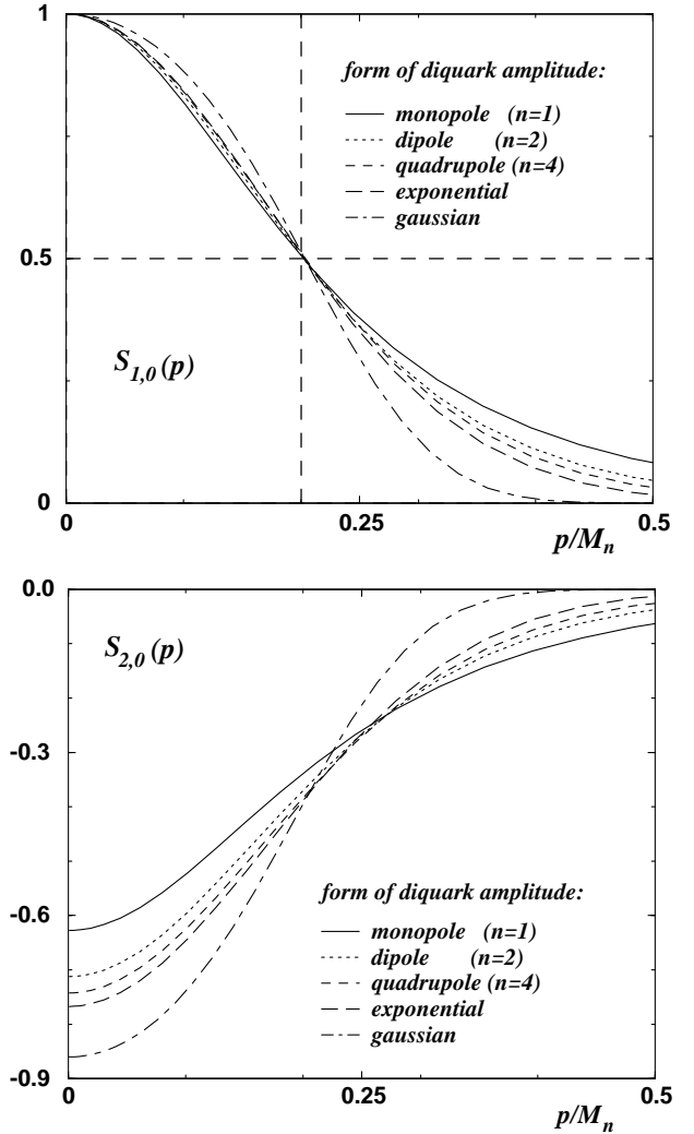
Fig. 5. The leading moments of the nucleon BS amplitudes S_1 (top) and S_2 (bottom) for the diquark amplitudes (2.15, 2.16) with m_q adjusted to yield S_{1,0}(p)|_{p=0.2M_n} = 1/2 .
