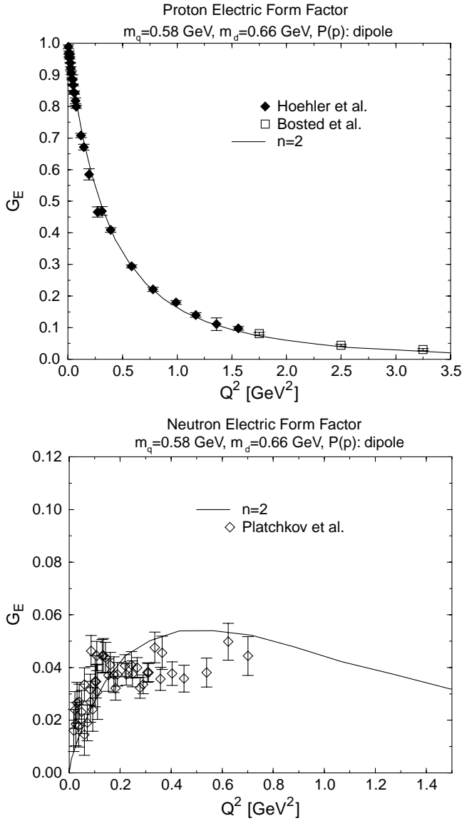
Fig. 11. Comparison of the electric form factors of proton and neutron with the experimental data of refs. [54,55] (top) and ref. [56] (bottom). Here, the dipole form of the diquark amplitude was used corresponding to the n = 2 result of fig. 10.
