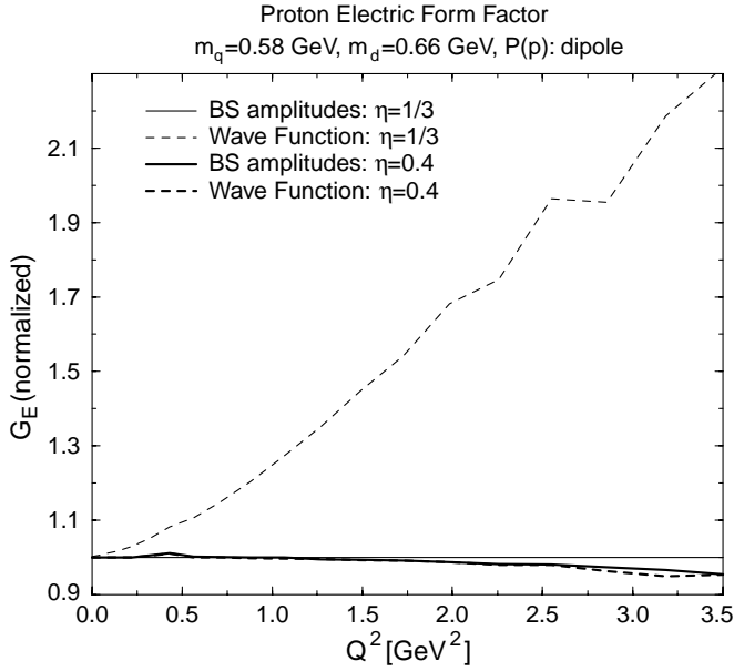
Fig. 17. The impulse-approximate contribution, corresponding to the diagrams of fig. 8, to the electric form factor of the proton (employing the dipole diquark amplitude). Results of the BS wave function calculations for the \eta -values 1/3 and 0.4 are compared to the respective amplitude plus residue calculations. The results are normalized to the latter with \eta = 1/3 .
