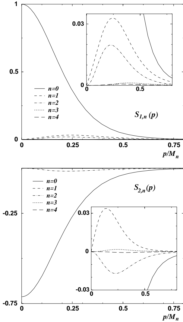
Fig. 3. The first 5 moments of the nucleon BS amplitudes S_1 (top) and S_2 (bottom).
