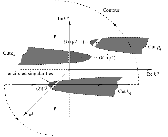
Fig. 16. Location of the relevant singularities in the impulse-approximate quark contribution to the form factors. The relative momentum k is the integration variable in the loop diagram corresponding to eq. (D.1).
