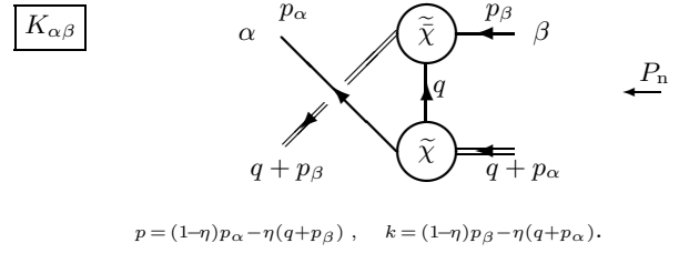
Fig. 2. The quark-exchange kernel of the nucleon BSE.
