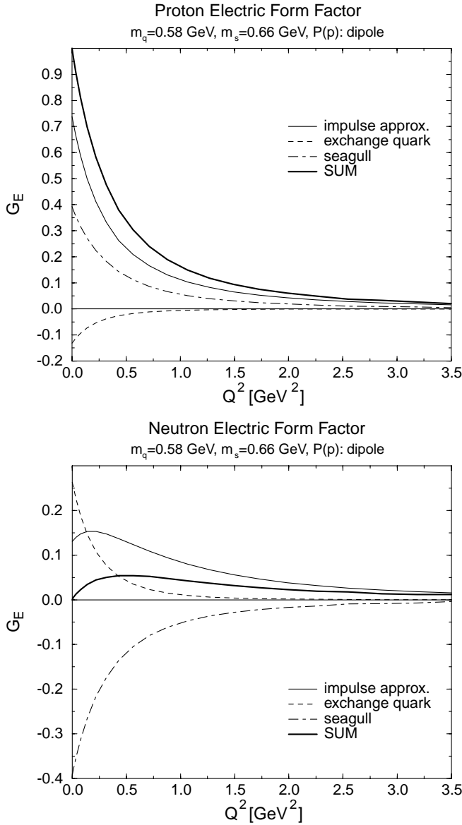
Fig. 13. Contribution of the single diagrams to neutron and proton electric form factors. The diquark amplitude is the dipole. The sum of these contributions (SUM) corresponds to the result of fig. 11.
