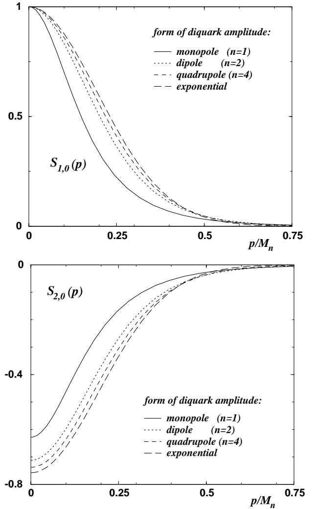
Fig. 6. The moments S_{1,0} (top) and S_{2,0} (bottom) of the nucleon amplitudes for the diquark amplitudes of eqs. (2.15,2.16) with fixed masses, m_s = 0.7M_n , m_q = 0.62M_n .
