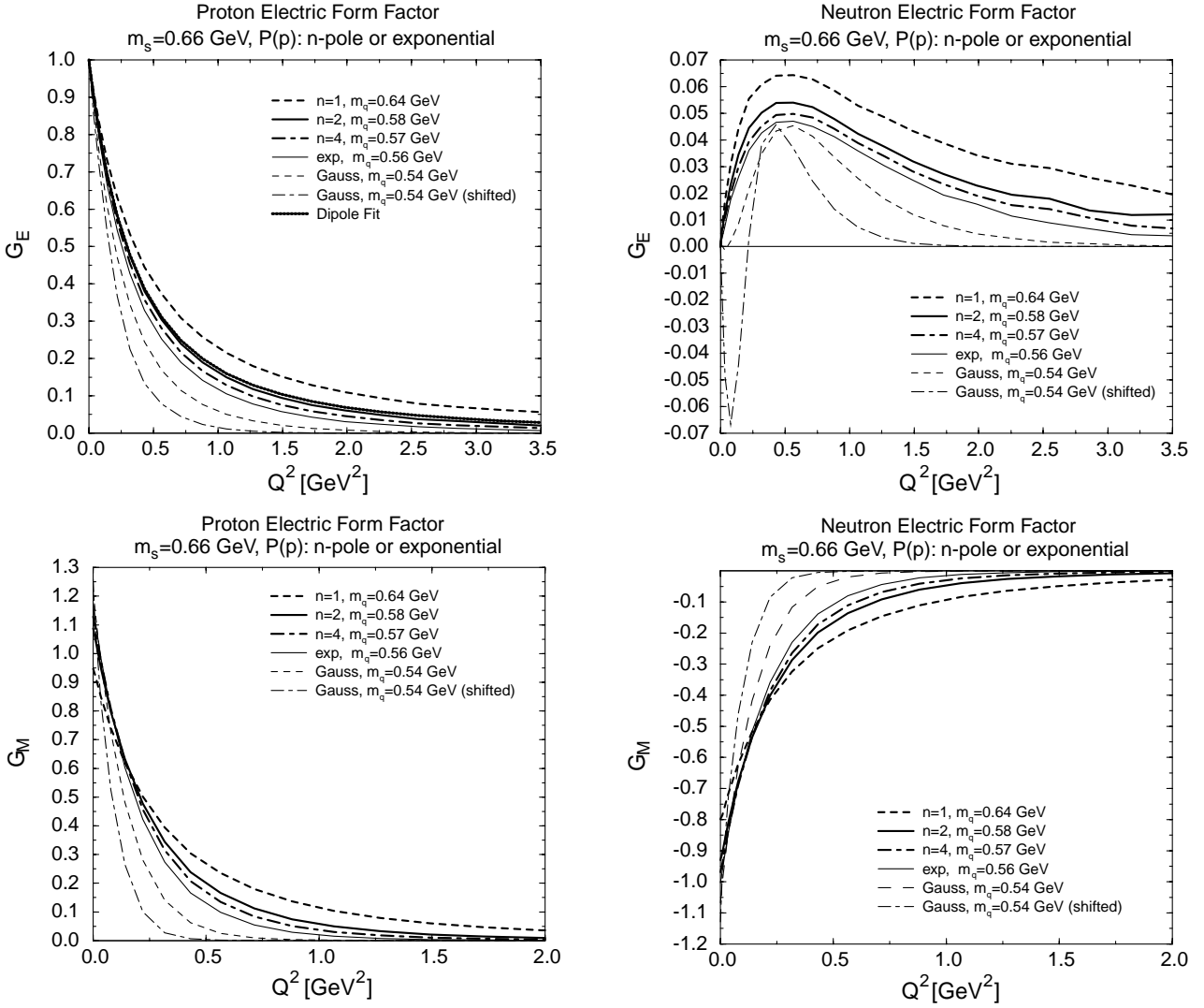
Fig. 10. Nucleon electric and magnetic form factors for fixed widths of S_{1,0} . The label Gauss, shifted refers to a calculation with diquark vertex function P_{\text{Gauss}} = \exp(-(p^2/\gamma_{\text{Gauss}} - 1)^2) . The parameters are listed in Tables 1 and 2 in sect. 3.
