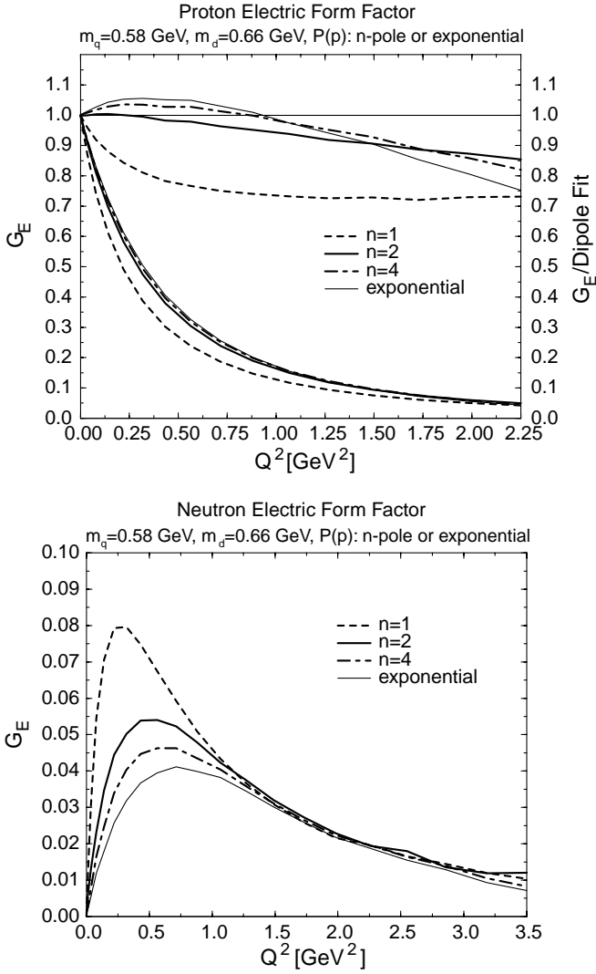
Fig. 12. Nucleon electric form factors for fixed quark and diquark masses. In the top plot, the bottom set of curves represent the results obtained for the proton electromagnetic form factor G_E(Q^2) and the top set of curves depict the ratios of these form factors over the dipole fit (1 + Q^2/(0.84 \text{ GeV})^2)^{-2} .
